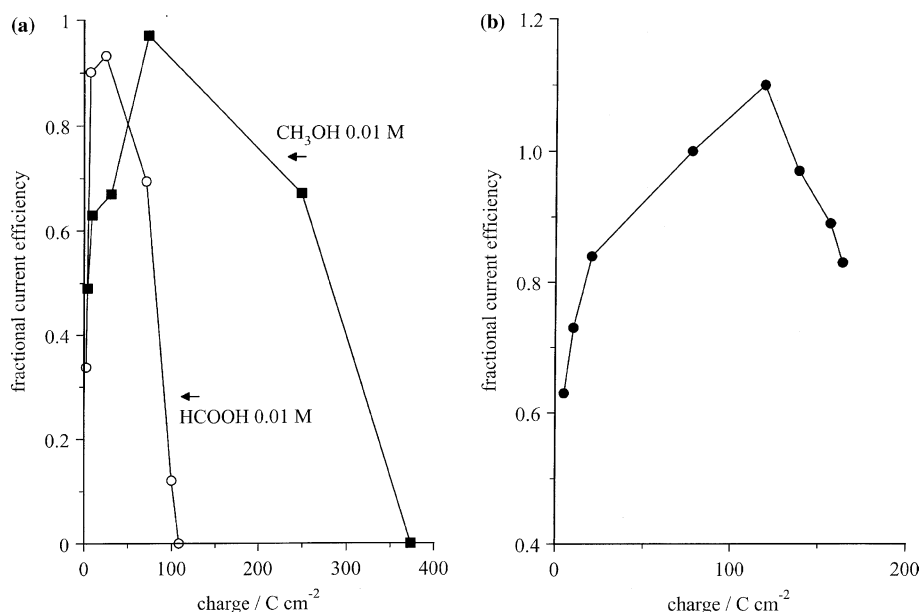
Fig. 5. Changes in the current efficiency observed during prolonged photoelectrolysis of 30 ml of 10^{-2} M solutions of (a) formic acid and methanol and (b) oxalic acid at a \text{WO}_3 film electrode under 1 sun AM 1.5 illumination. 1 M \text{NaHSO}_4(\text{aq}) (pH 2) was the supporting electrolyte. Applied bias voltage 1 V. The current yields were derived from the amount of formed \text{CO}_2 and are plotted against the amount of electric charge.
